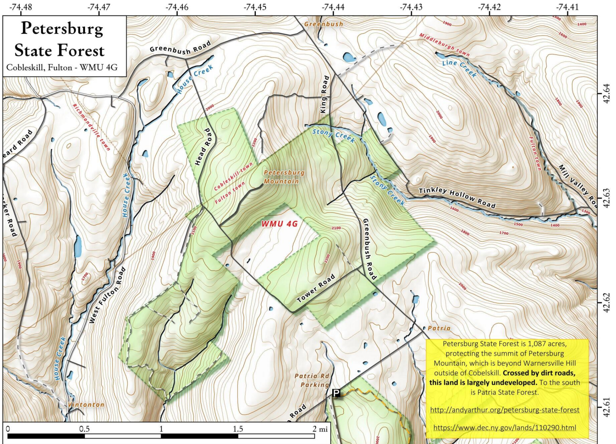
Petersburg State Forest Map, August 18, 2018 by AndyArthur.org in QGIS 3.2.1-Bonn and Python. Street Map is Copyright © OpenStreetMap contributors, CC BY-SA. NYSDEC Data: LiDAR/DEM, Borders, ADK Wetlands, Trails, Assets. True North. 1 inch = 0.4 miles. Projection: NAD83 / UTM zone 18N. Coordinates: 0.01° latitude-longitude (WGS84). Contours are 20 feet.
