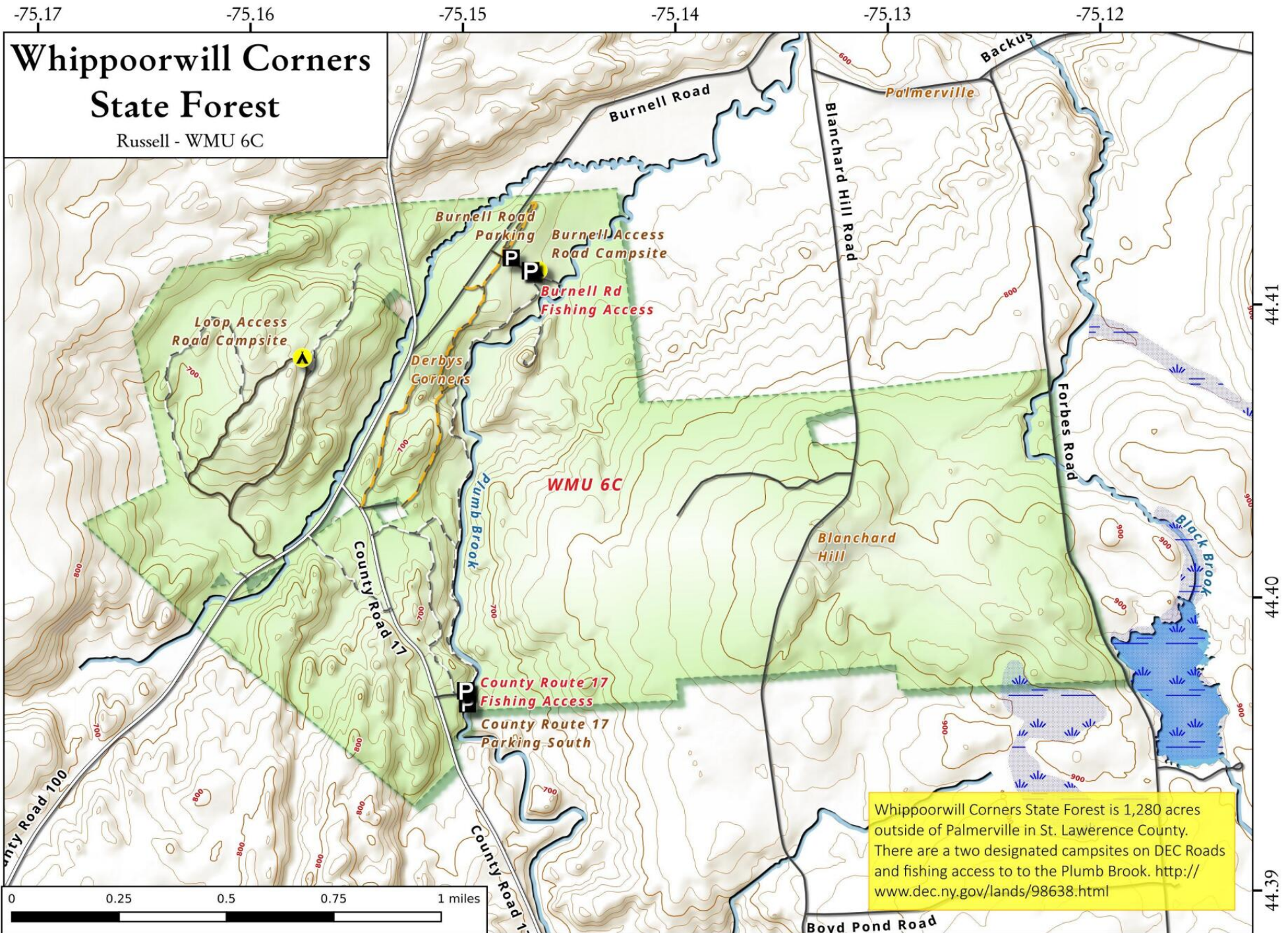
Whippoorwill Corners State Forest Map, June 28, 2018 by AndyArthur.org in QGIS 3.0.3-Girona and Python. Street Map is Copyright © OpenStreetMap contributors, CC BY-SA. NYSDEC Data: LiDAR/DEM, Borders, ADK Wetlands, Trails, Assets. True North. 1 inch = 0.3 miles. Projection: NAD83 / UTM zone 18N. Coordinates: 0.01° latitude-longitude (WGS84). Contours are 20 feet.
