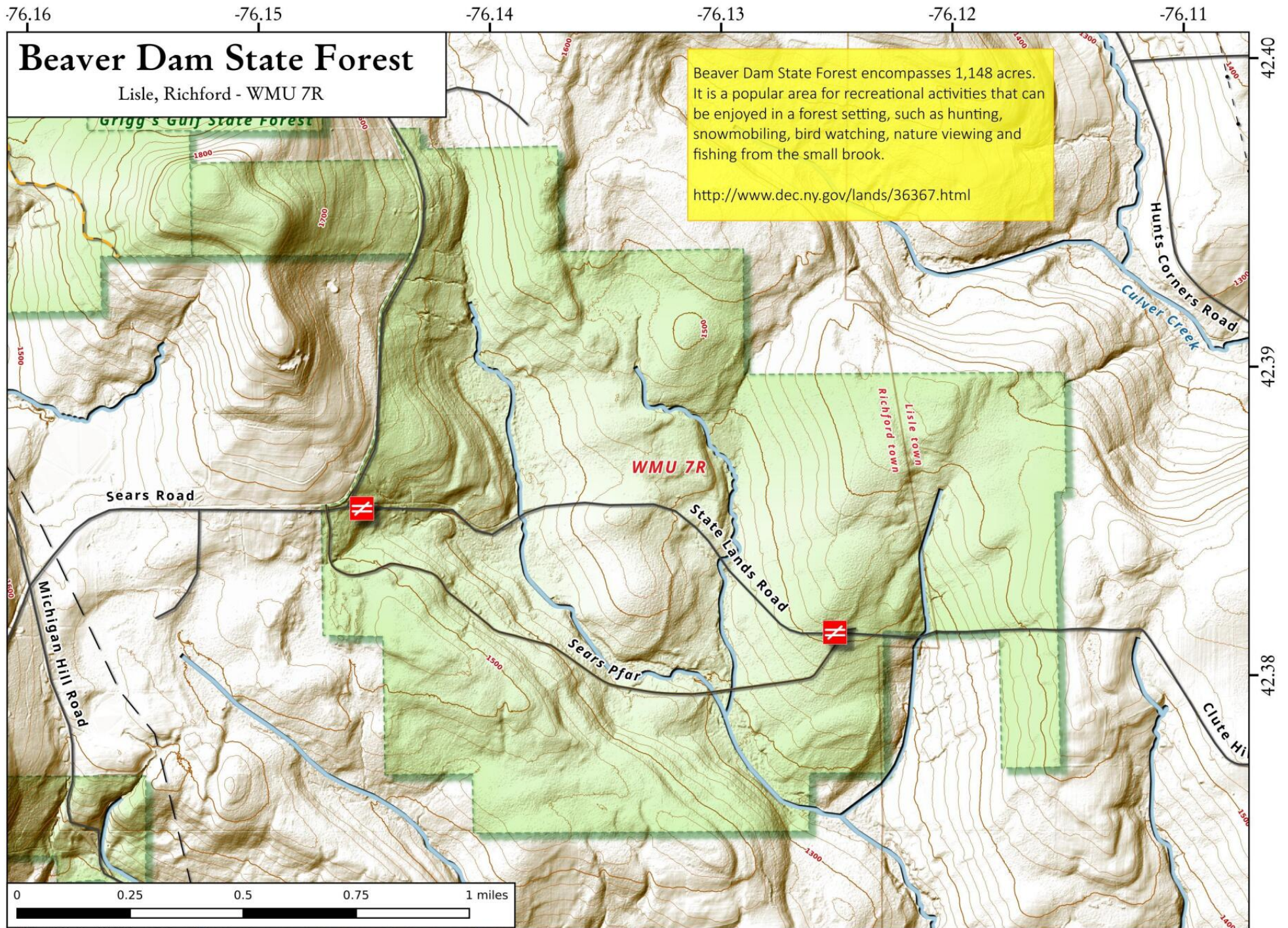
Beaver Dam State Forest Map, April 27, 2018 by AndyArthur.org in QGIS 3.0.1-Girona and Python. Street Map is Copyright © OpenStreetMap contributors, CC BY-SA. NYSDEC Data: LiDAR, Borders, ADK Wetlands, Trails, Assets. True North. 1 inch = 0.3 miles. Projection: NAD83 / UTM zone 18N. Coordinates: 0.01° latitude-longitude (WGS84). Contours are 10 feet.
