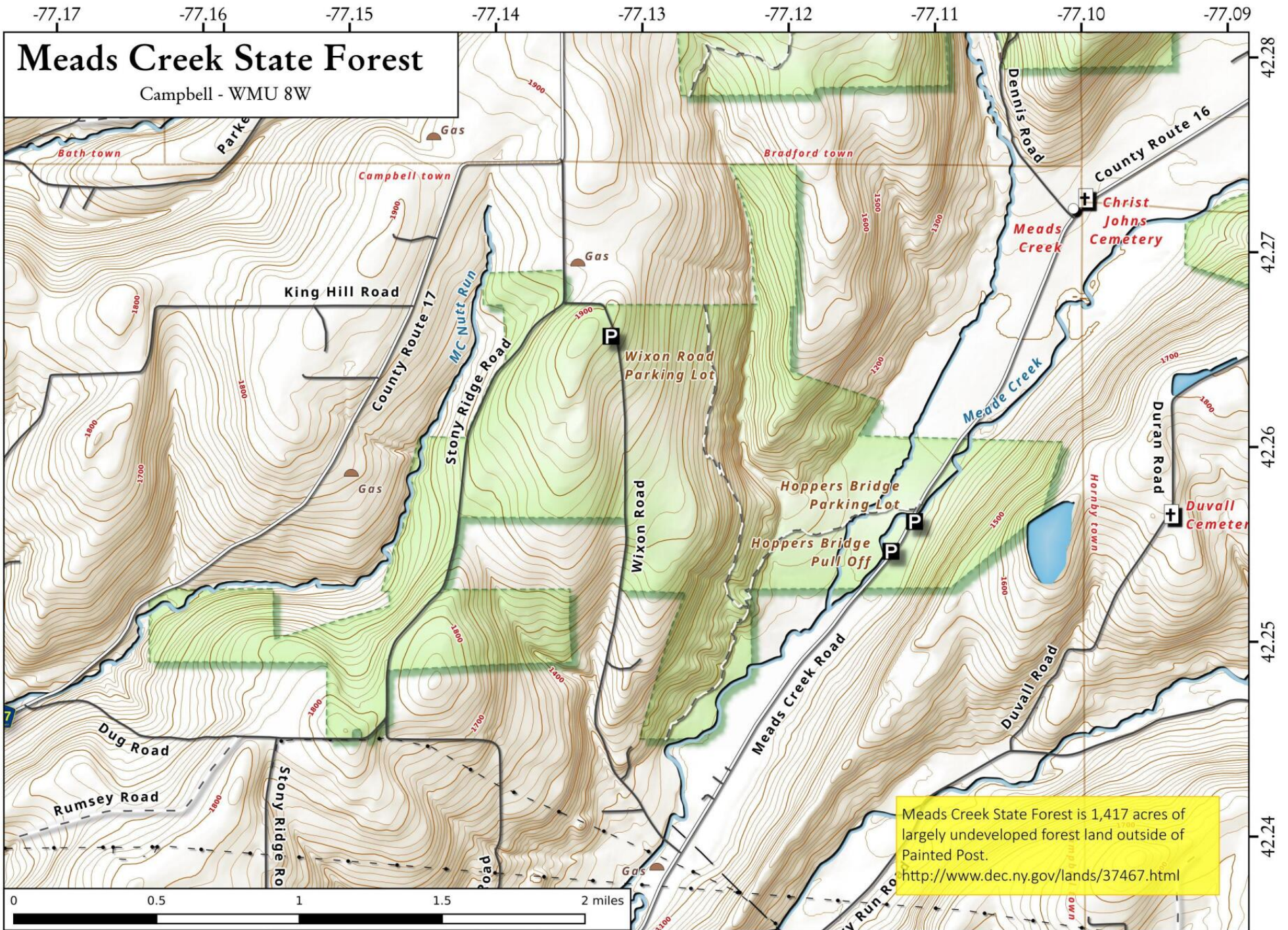
Meads Creek State Forest Map, April 8, 2018 by AndyArthur.org in QGIS 3.0.1-Girona and Python. Street Map is Copyright © OpenStreetMap contributors, CC BY-SA. NYSDEC Data: LiDAR/DEM, Borders, ADK Wetlands, Trails, Assets. True North. 1 inch = 0.3 miles. Projection: NAD83 / UTM zone 18N. Coordinates: 0.01° latitude-longitude (WGS84). Contours are 20 feet.
